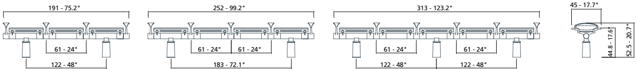
Backless seat with armrest
