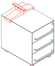
Support for structural pedestal (Nomos-side return) 1BA1551
