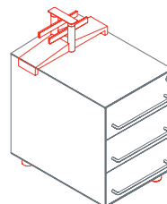
Support for structural pedestal (Nomos desk) 1B1541
