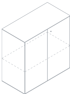
Cabinet with lockable door (1 shelf included) 1BA6070: L 31½ D 17¾ H 28¾ 1BA6075: L 31½ D 17¾ H 39½
