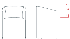
Tall armchair on feet 1PL6012: L 56 D 50,5 H 75
