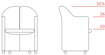
Tall armchair on castors 1PS6021: L 22 1/2 D 22 H 32 1/4
