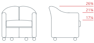
Armchair on castors 1PS6011: L 26 3/4 D 23 3/4 H 26 3/4
