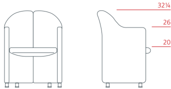
Tall armchair on feet 1PS6022: L 22 1/2 D 22 H 32 1/4
