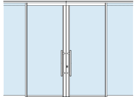
Framed double sliding door in single laminated transparent glass.
